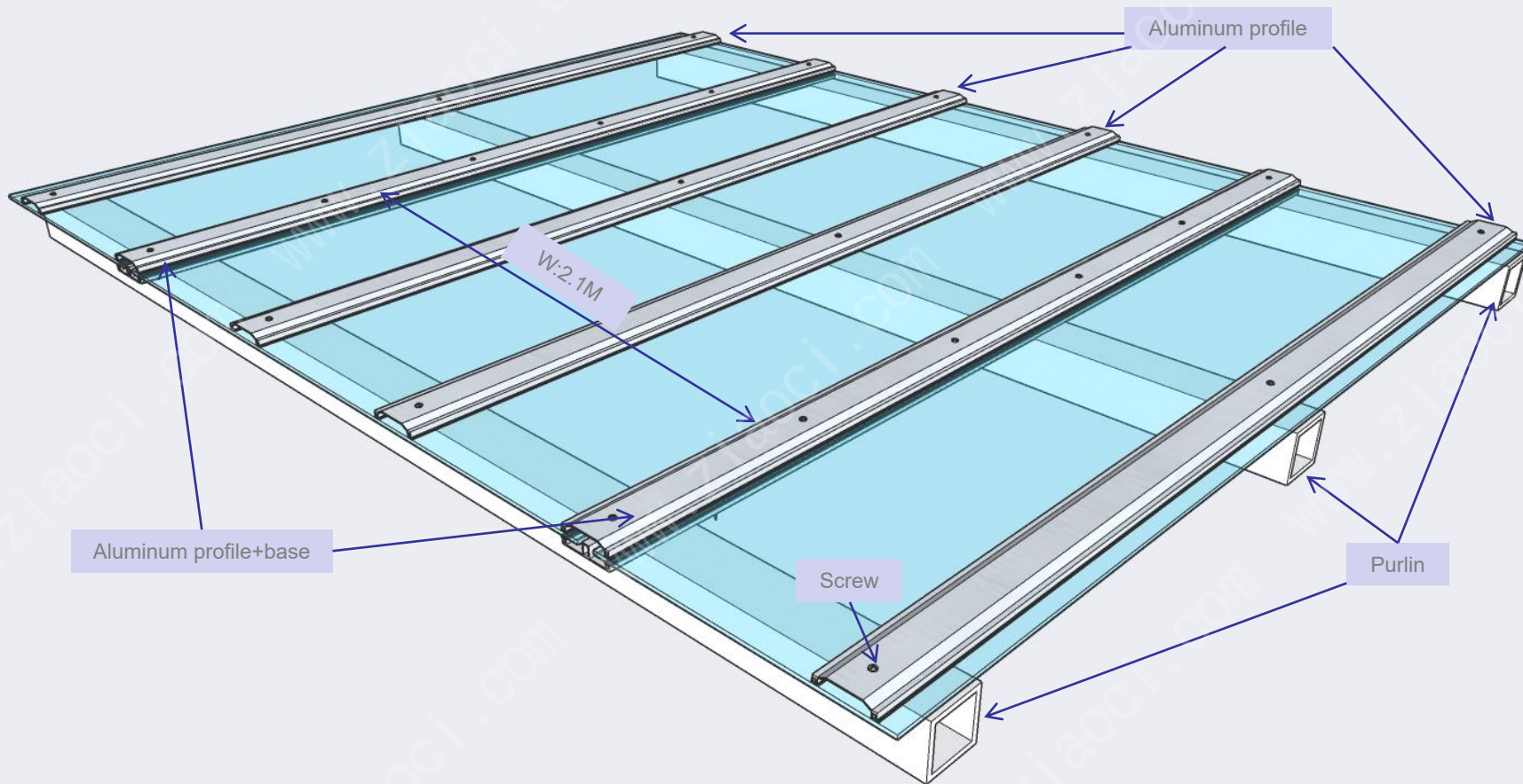
PC hollow sheet canopy - Structural Diagram
