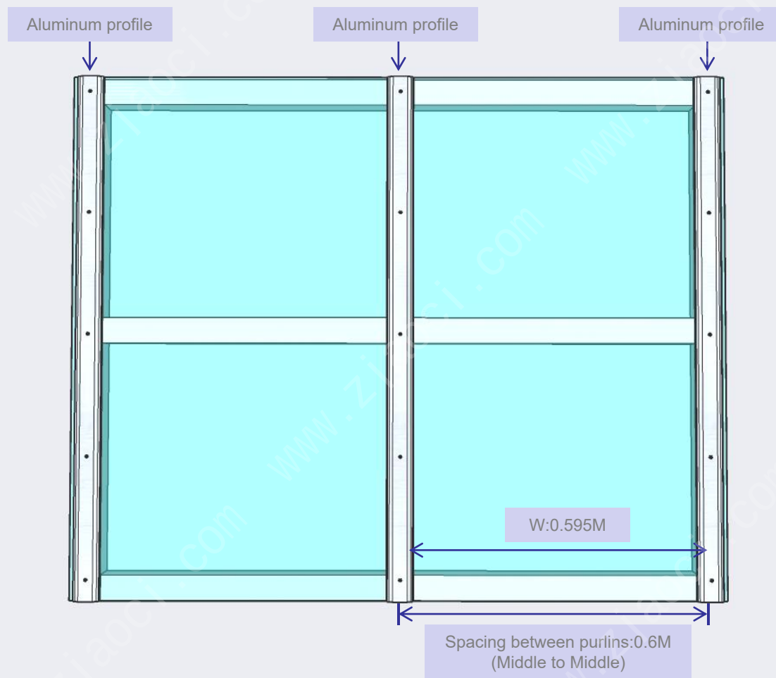
PC solid sheet canopy - Vertical View
