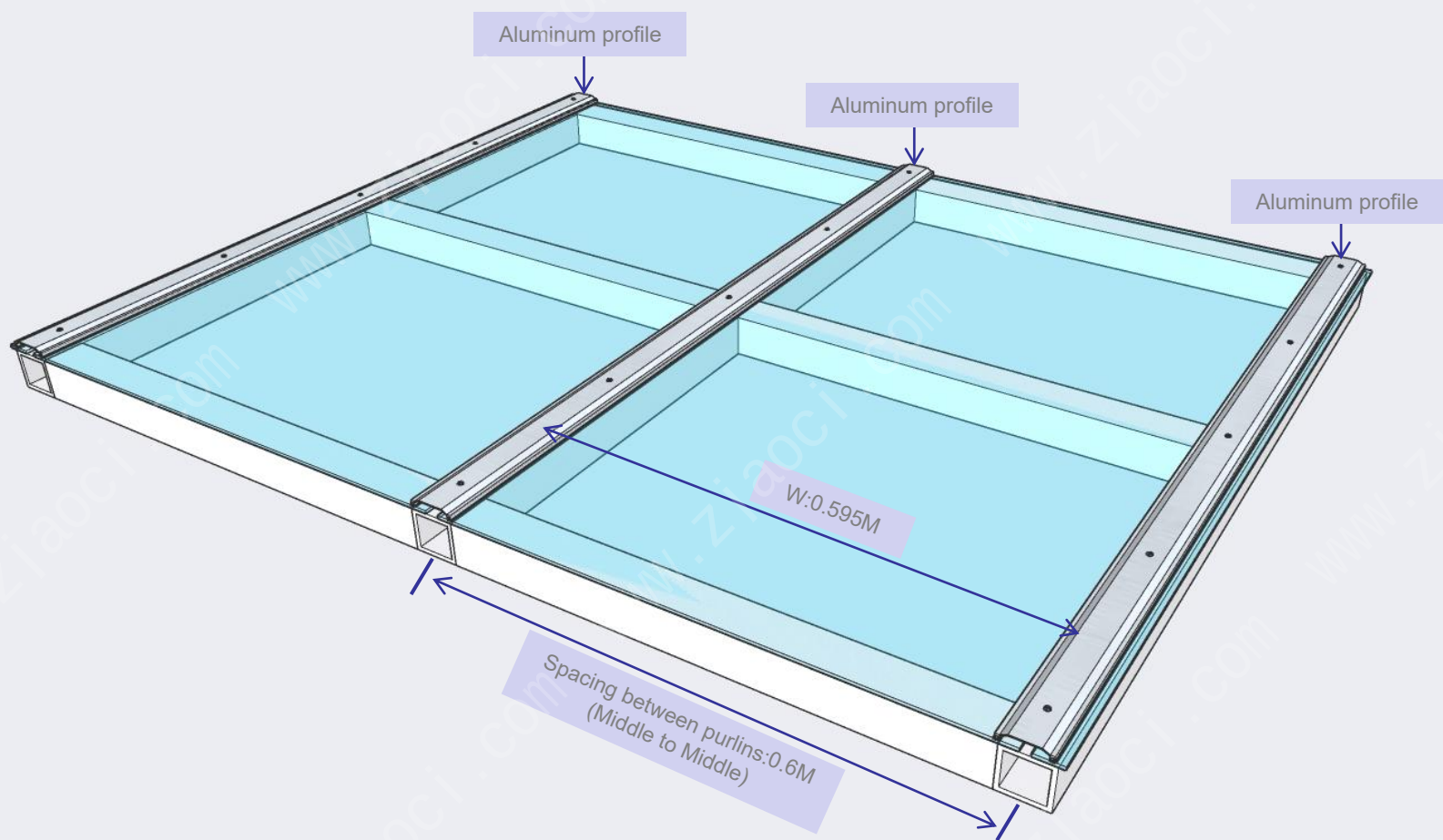
PC solid sheet canopy - Structural Diagram
