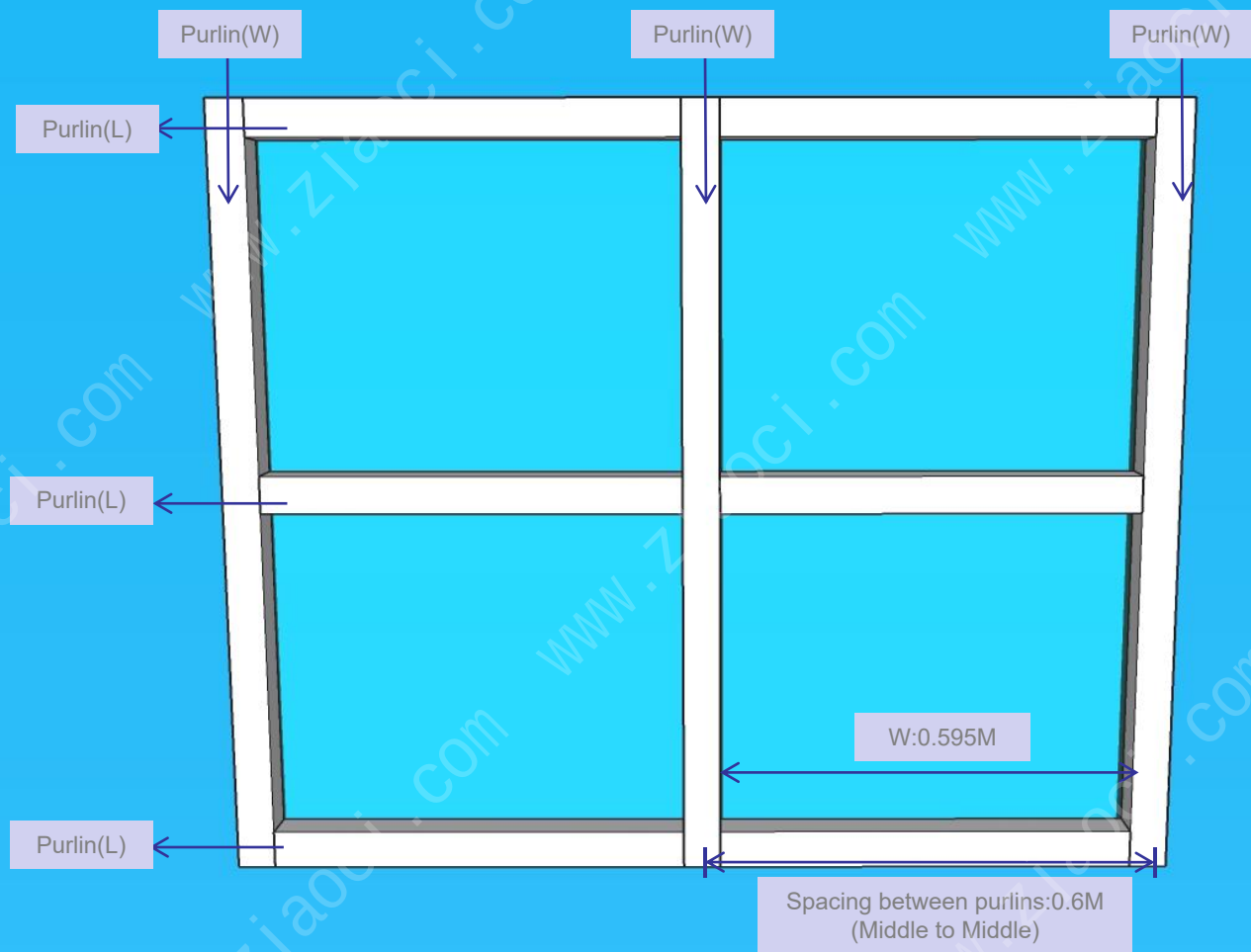
PC solid sheet canopy - Bottom View
