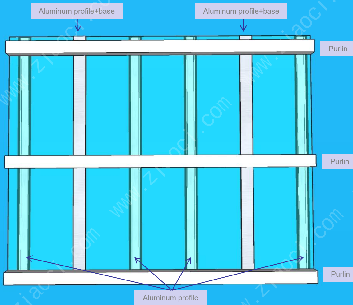
PC hollow sheet canopy - Bottom View
